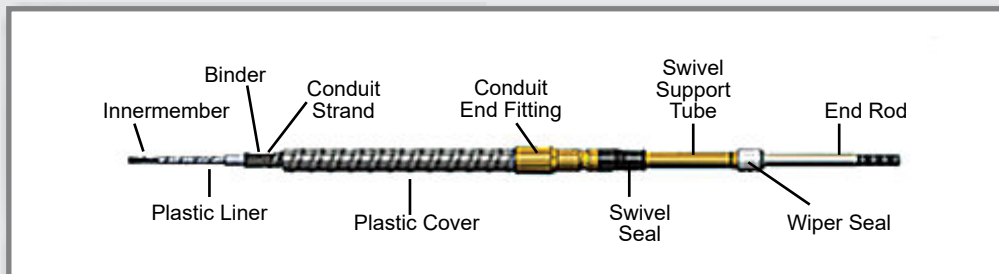
Push-Pull Cable
