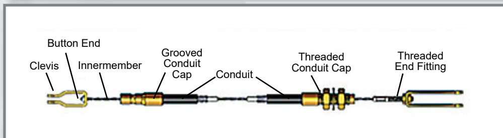
Pull-Only Brake Cable
